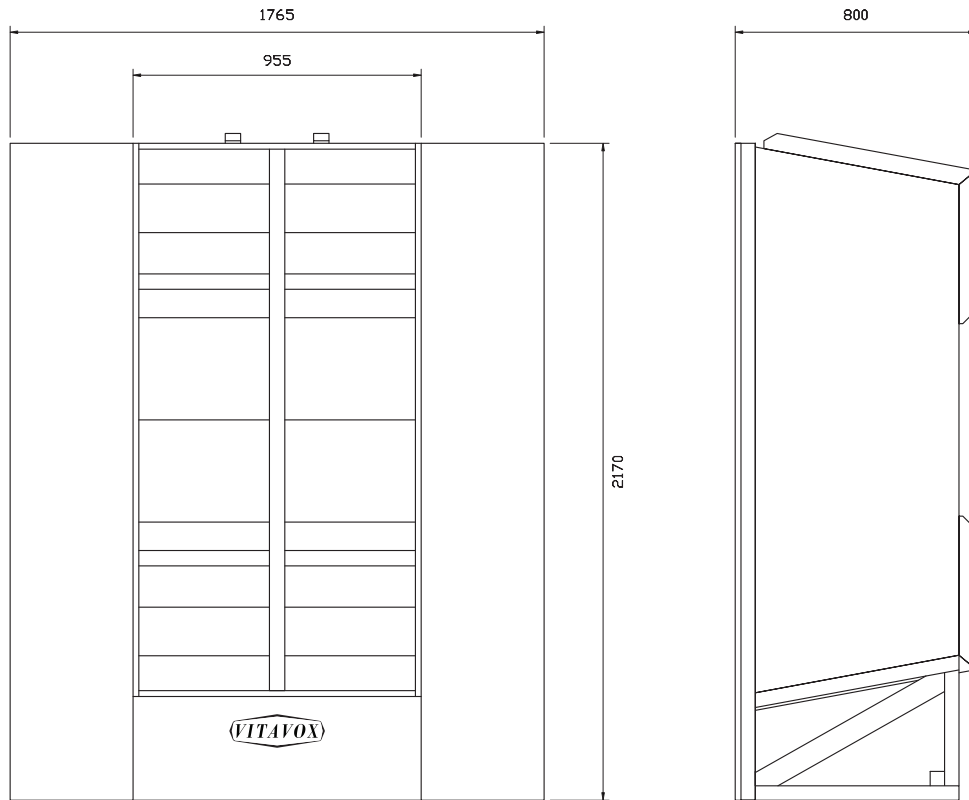
BASS BIN (SHOWN WITH OPTIONAL SIDE BAFFLES)
